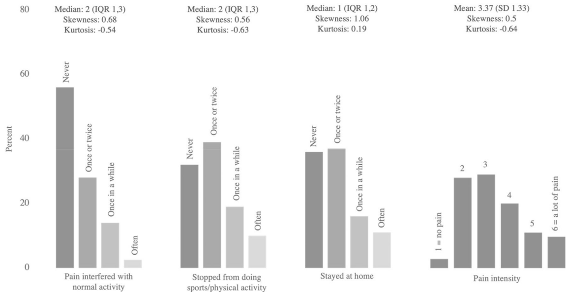
Fig. 1 Histogram of each item.
